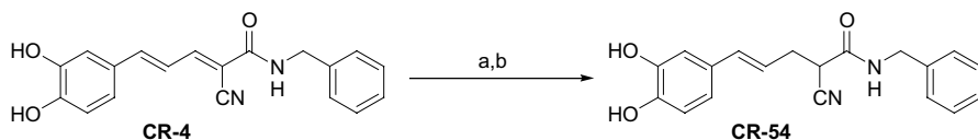
Scheme 4. Reagents and conditions: (a) \text{NaBH}_4 , MeOH, 1 h, 20 °C; (b) HPLC, Nova-Pak C18 19.0×300 mm, gradient MeCN–H 2 O, 20:80 \rightarrow MeCN–H 2 O, 80:20.
