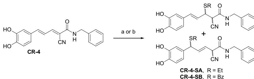
Scheme 5. Reagents and conditions: (a) EtSH, DMSO, piperidine, 0.5 h, 20 °C; (b) BzSH, DMSO, 0.5 h, 20 °C.
