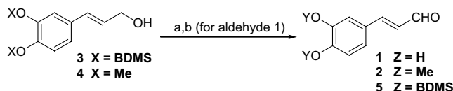
Scheme 2. Reagents and conditions: (a) activated MnO_2 , CH_2Cl_2 ; (b) n -Bu 4 NF, CHCl_3 .
