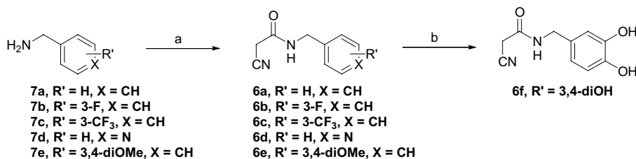
Scheme 3. Reagents and conditions: (a) \text{N}\equiv\text{CCH}_2\text{COOMe} neat, 2 h, 20 °C; (b) 9e , \text{BBr}_3 , \text{CH}_2\text{Cl}_2 , -78^\circ\text{C} \rightarrow 20^\circ\text{C} .
