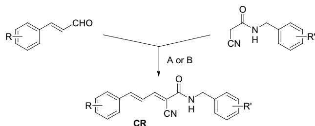
Scheme 1. Reagents and conditions: (A) piperidine, EtOH, 0.5 h, 20 °C (when R = OH); (B) \beta -alanine, EtOH, 80 °C, 1–4 h (when R \neq OH).
